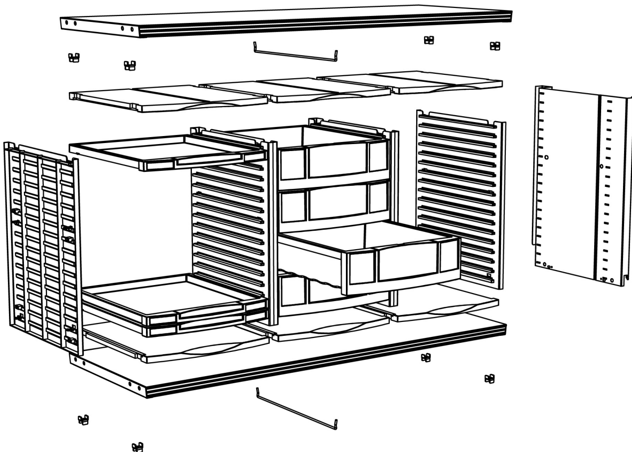
Exploded view
