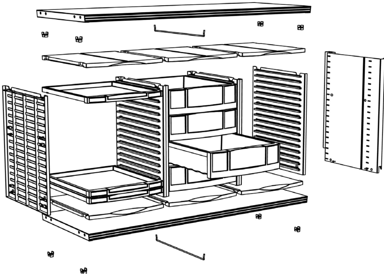
Exploded view
